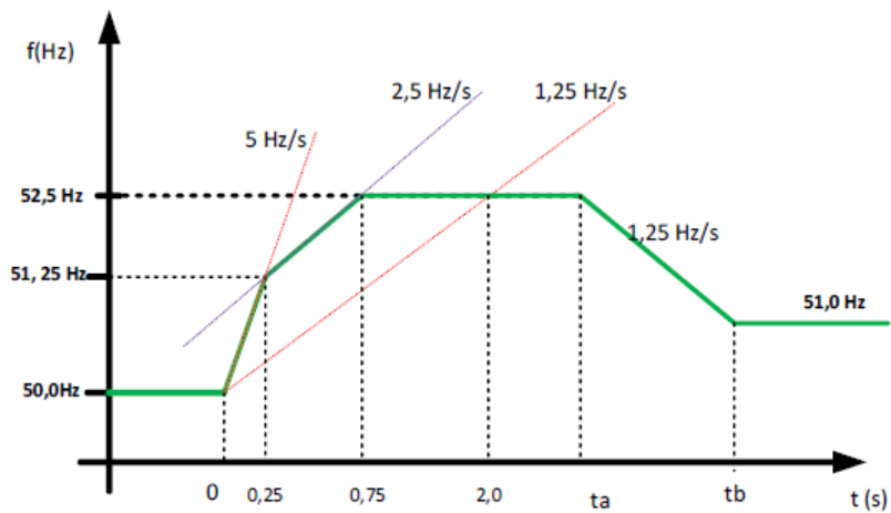
Figure X-a: The frequency ride through profile that an HVDC system should remain connected to the network for the case of over-frequency. The value t_a and t_b shall be specified by the relevant TSO, but longer than for A-PPMs according to Article 39.
