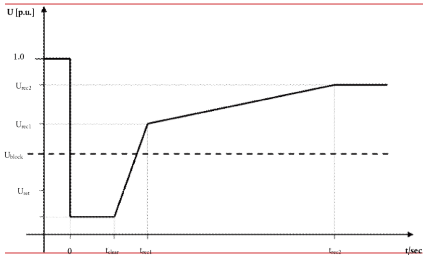
Figure 6: Fault-ride-through profile of an HVDC converter station. The diagram represents the lower limit of a voltage- against-time profile at the connection point, expressed by the ratio of its actual value and its reference 1 pu value in per unit before, during and after a fault. U prefault is the pre-fault voltage. U ret is the retained voltage at the connection point during a fault, t clear is the instant when the fault has been cleared, U rec1 and t rec1 specify a point of lower limits of voltage recovery following fault clearance. U block is the blocking voltage at the connection point. The time values referred to are measured from t fault .
