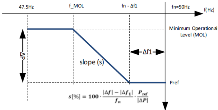
Figure X-c: LFSM-UC curve for a power-to-gas demand unit
