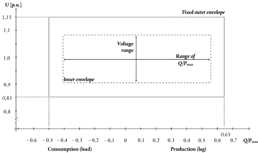
Figure 7: U-Q/Pmax-profile of an DC-asynchronously connected power park module and asynchronously connected electricity storage module at the connection point. The diagram represents boundaries of a U-Q/Pmax-profile of the voltage at the connection point[s], expressed by the ratio of its actual value to its reference 1 pu value in per unit, against the ratio of the reactive power (Q) to the maximum capacity (Pmax). The position, size and shape of the inner envelope are indicative and other than rectangular may be used within the inner envelope. For profile shapes other than rectangular, the voltage range represents the highest and lowest voltage points. Such a profile would not give rise to the full reactive power range being available across the range of steady-state voltages.
