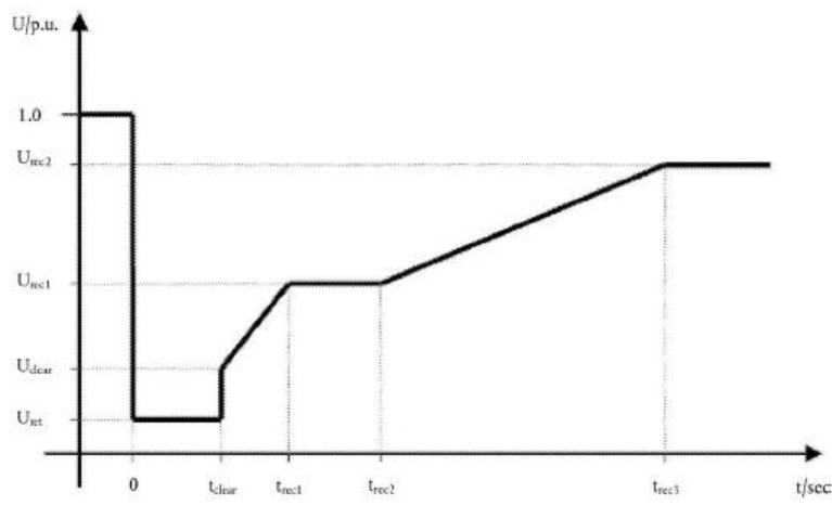
Figure X-d: Fault-ride-through profile of a Power-to-Gas Demand Unit.
