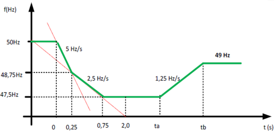
Figure X-b: The frequency ride through profile than an HVDC system should remain connected to the network for the case of under-frequency. The value t_a and t_b shall be specified by each relevant TSO, but longer than for A-PPMs according to Article 39.
