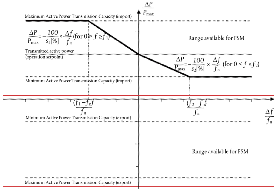
Figure 1: Active power frequency response capability of an HVDC system in FSM illustrating the case of zero with deadband and insensitivity with a positive active power setpoint (import mode). In this figure, \Delta P is the change in active power output from the change by an HVDC system with the network at its connection point based on its actual operating point, P_{max} is maximum transmission capacity of the HVDC system, f_n is the target frequency in the AC network where the FSM service is provided, and \Delta f is the frequency deviation in the AC network where the FSM service is provided, \Delta P1 is the agreed power change for the FSM at reaching the frequency threshold value \Delta f1 , \Delta P2 is the agreed power change at reaching the frequency threshold value \Delta f2 , \Delta f_{db} is the deadband of the power frequency response, \Delta f_{insensitivity} is the frequency response insensitivity (or else the permissible tolerance allowed), s1 is the droop value for the given \Delta P1 and s2 is the droop for the given \Delta P2 .
