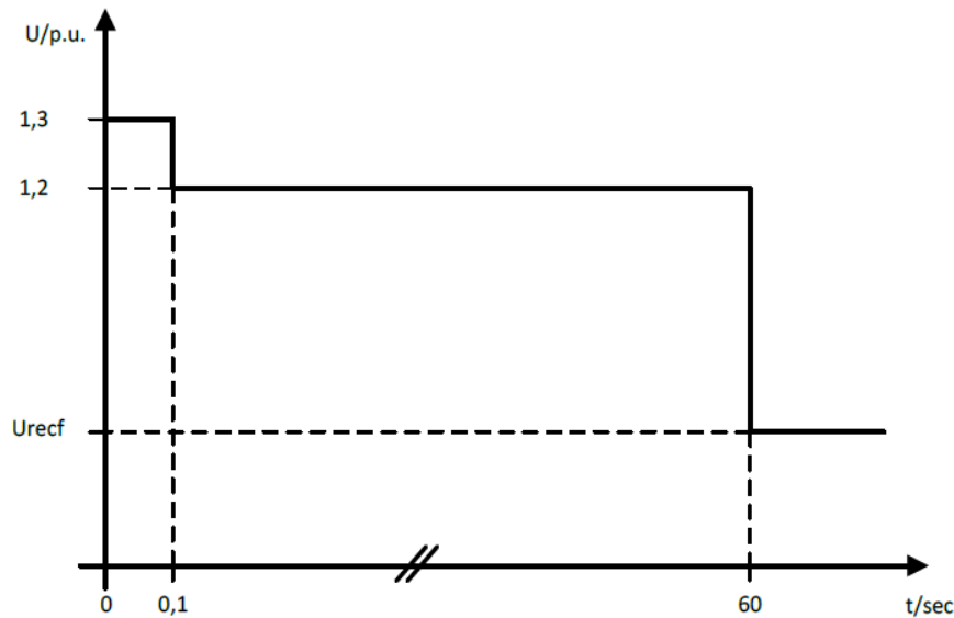
Figure Y-a: Overtoltage against-time profile of an A-PtG-DU. The diagram represents the higher limit of a voltage-against-time profile of the voltage at the isolated interface point, expressed as the ratio of its actual value and its reference 1 pu value, before, during and after a fault. Urefc is the maximum voltage as specified by the relevant TSO.
