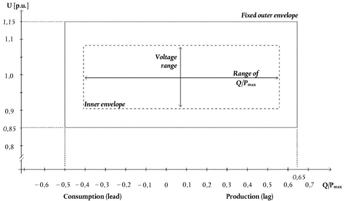
Figure 7: U-Q/Pmax-profile of an DC-connected power park module A-PPM and A-ESM at the connection point. The diagram represents boundaries of a U-Q/Pmax-profile of the voltage at the connection point[s], expressed by the ratio of its actual value to its reference 1 pu value in per unit, against the ratio of the reactive power (Q) to the maximum capacity (Pmax). The position, size and shape of the inner envelope are indicative and other than rectangular may be used within the inner-fixed outer envelope. For profile shapes other than rectangular, the voltage range represents the highest and lowest voltage points. Such a profile would not give rise to the full reactive power range being available across the range of steady-state voltages.
