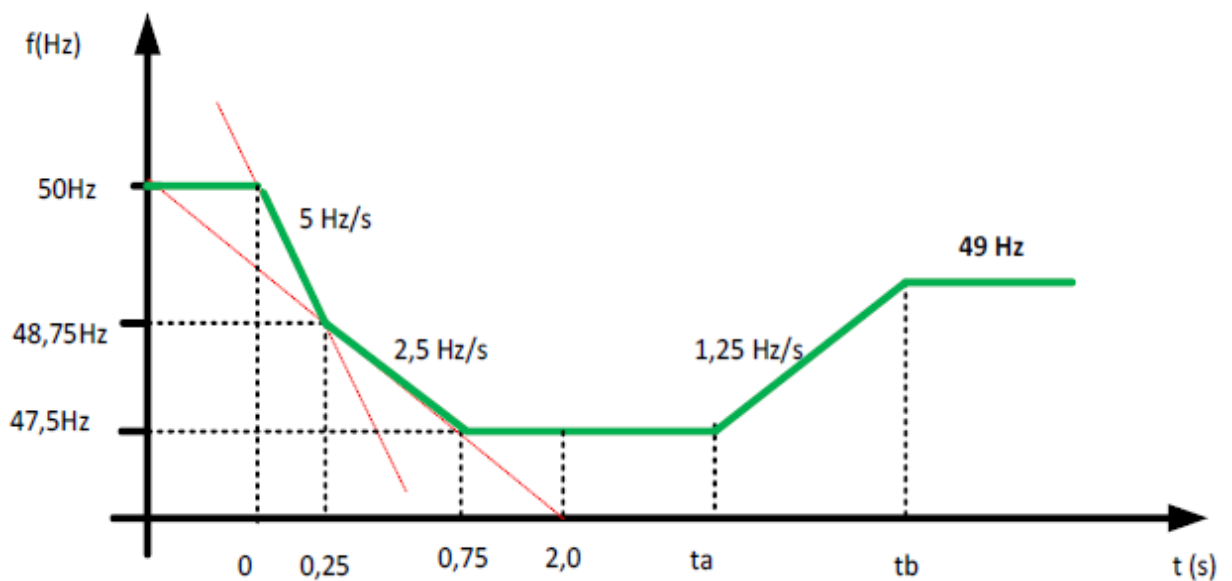
Figure X-b: The frequency ride through profile that an HVDC system shall remain connected to the network for the case of under-frequency. The value t_a and t_b shall be specified by each relevant TSO, but longer than for A-PPMs according to Article 39.
